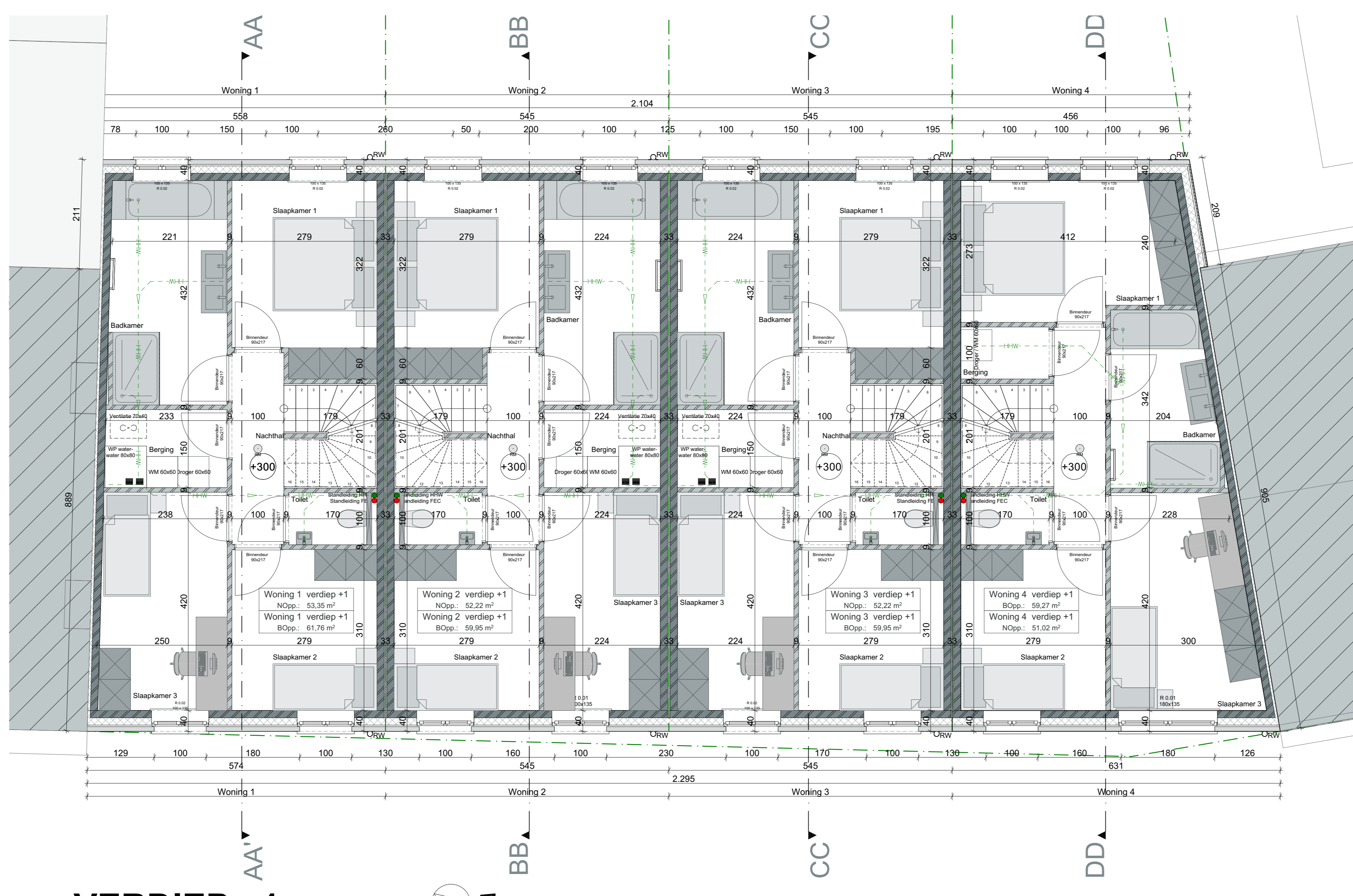
plan VERDIEP +1 1/50
