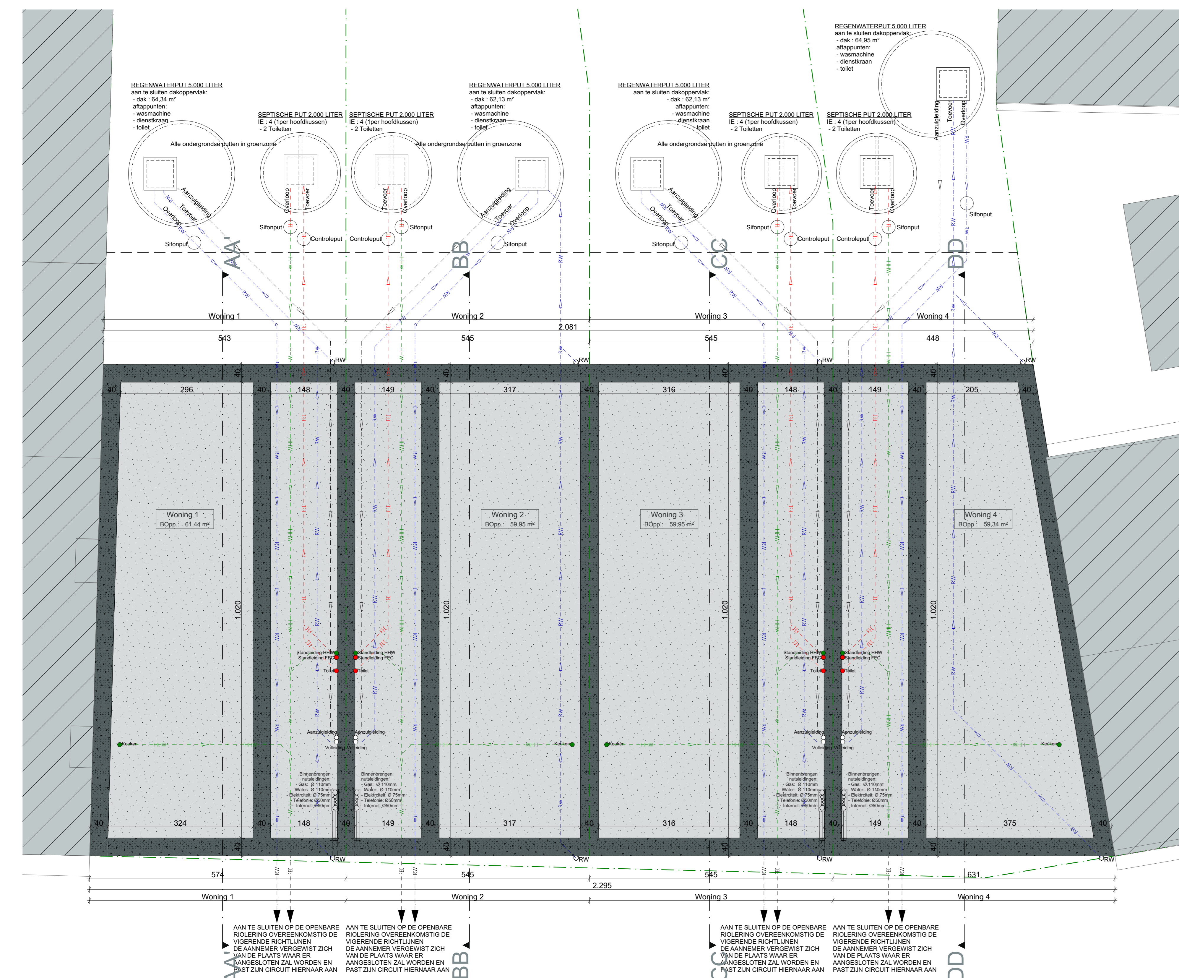
plan FUNDERING 1/50
