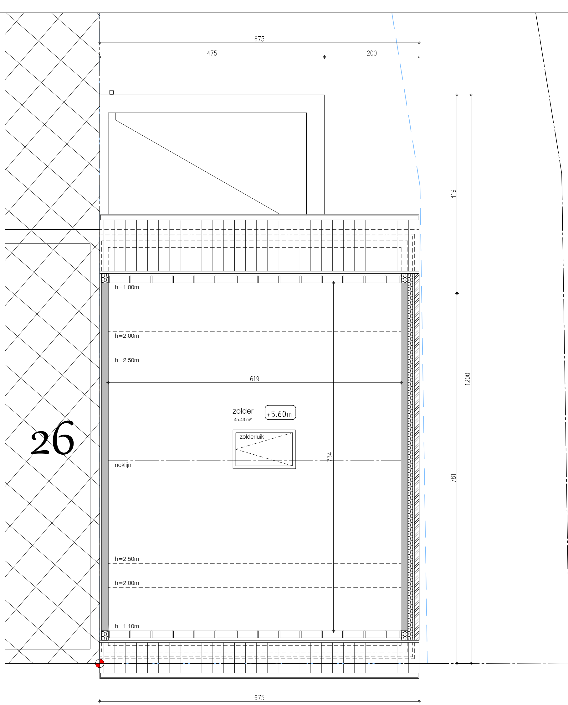
zolder lot 1
