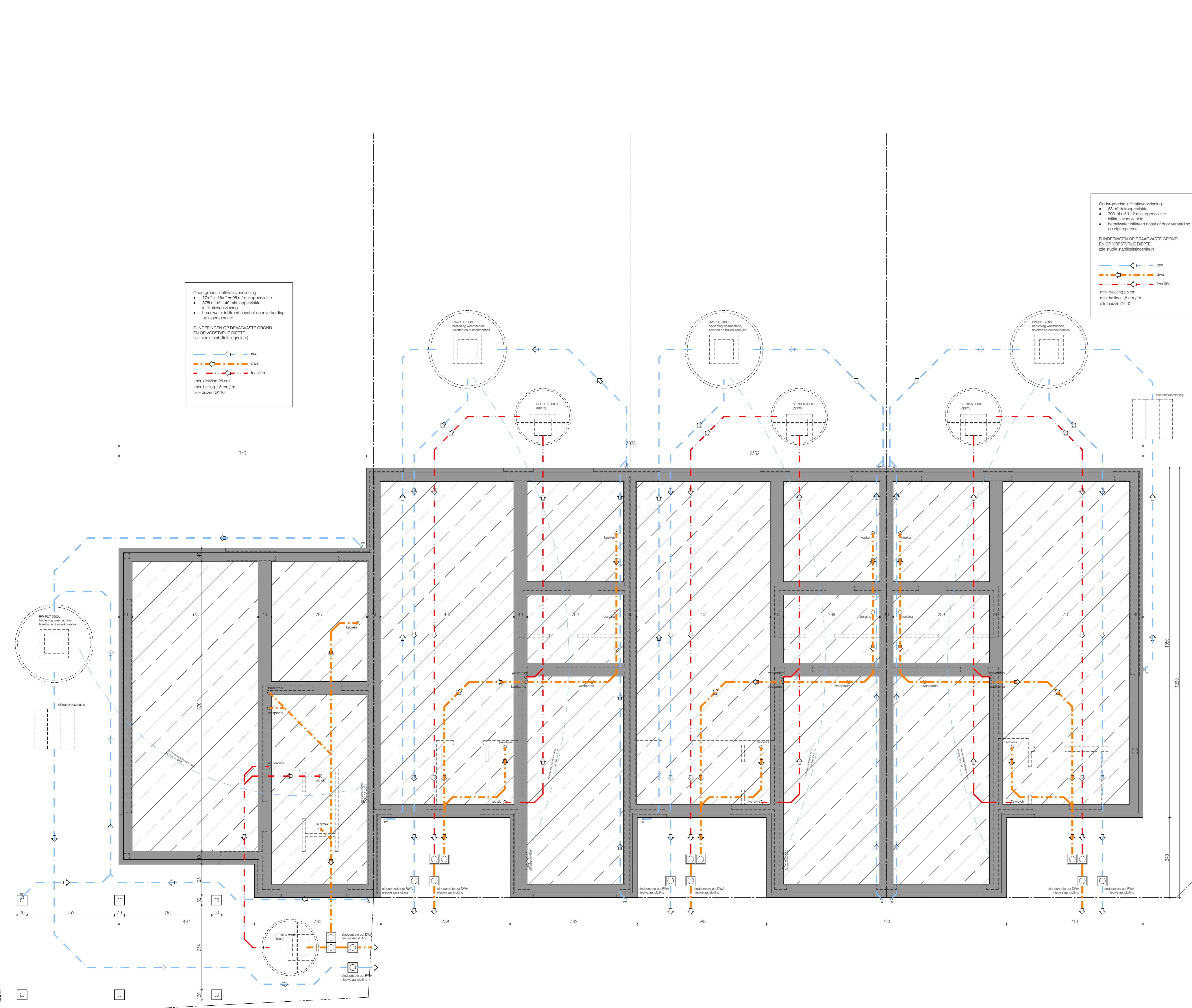
funderings- en rioleringsplan lot 15 76.23 m 2 bruto opp.
