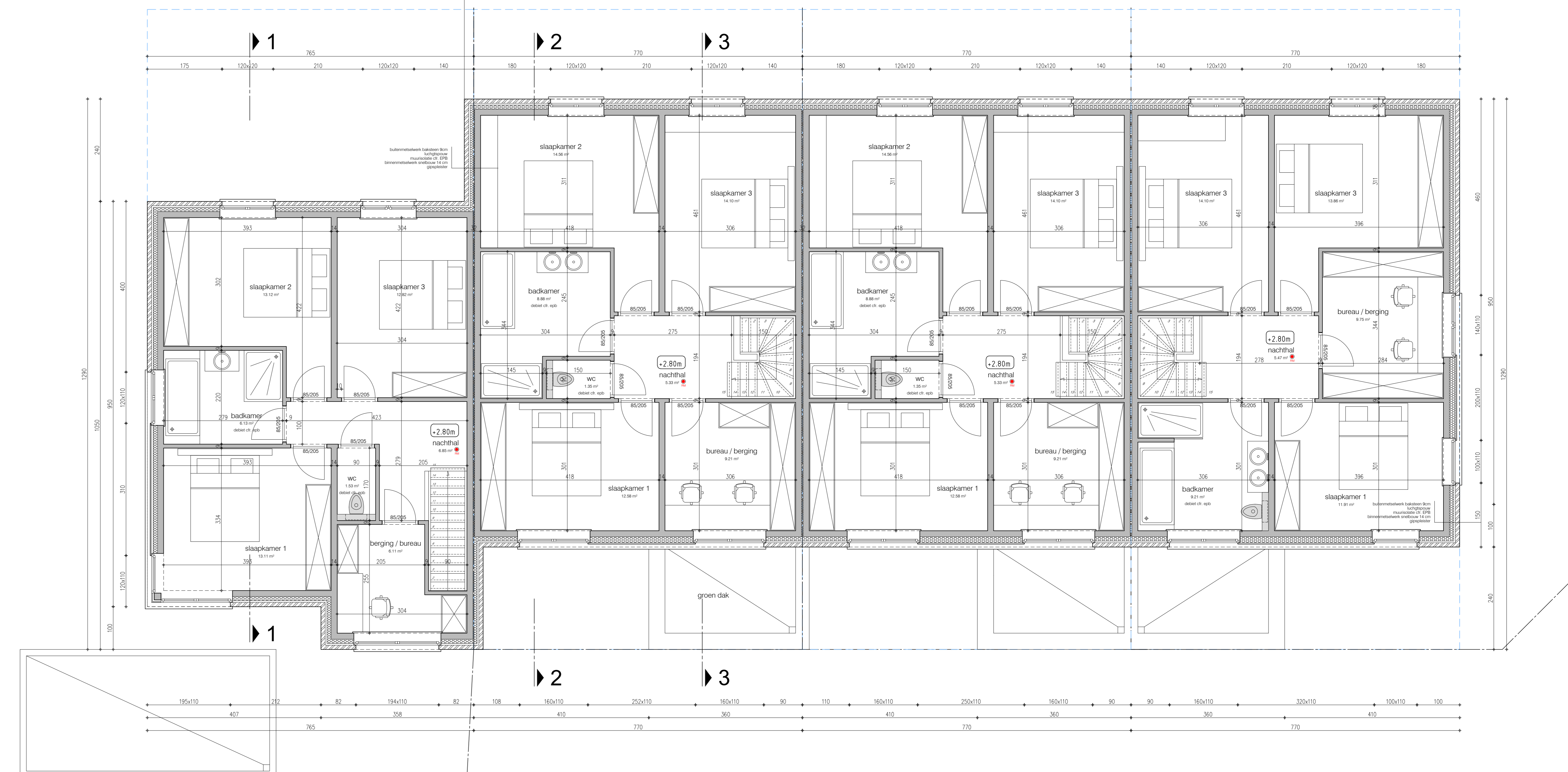
verdiepingsplan lot 15 76.23 m 2 bruto opp. 65.16 m 2 netto opp.
