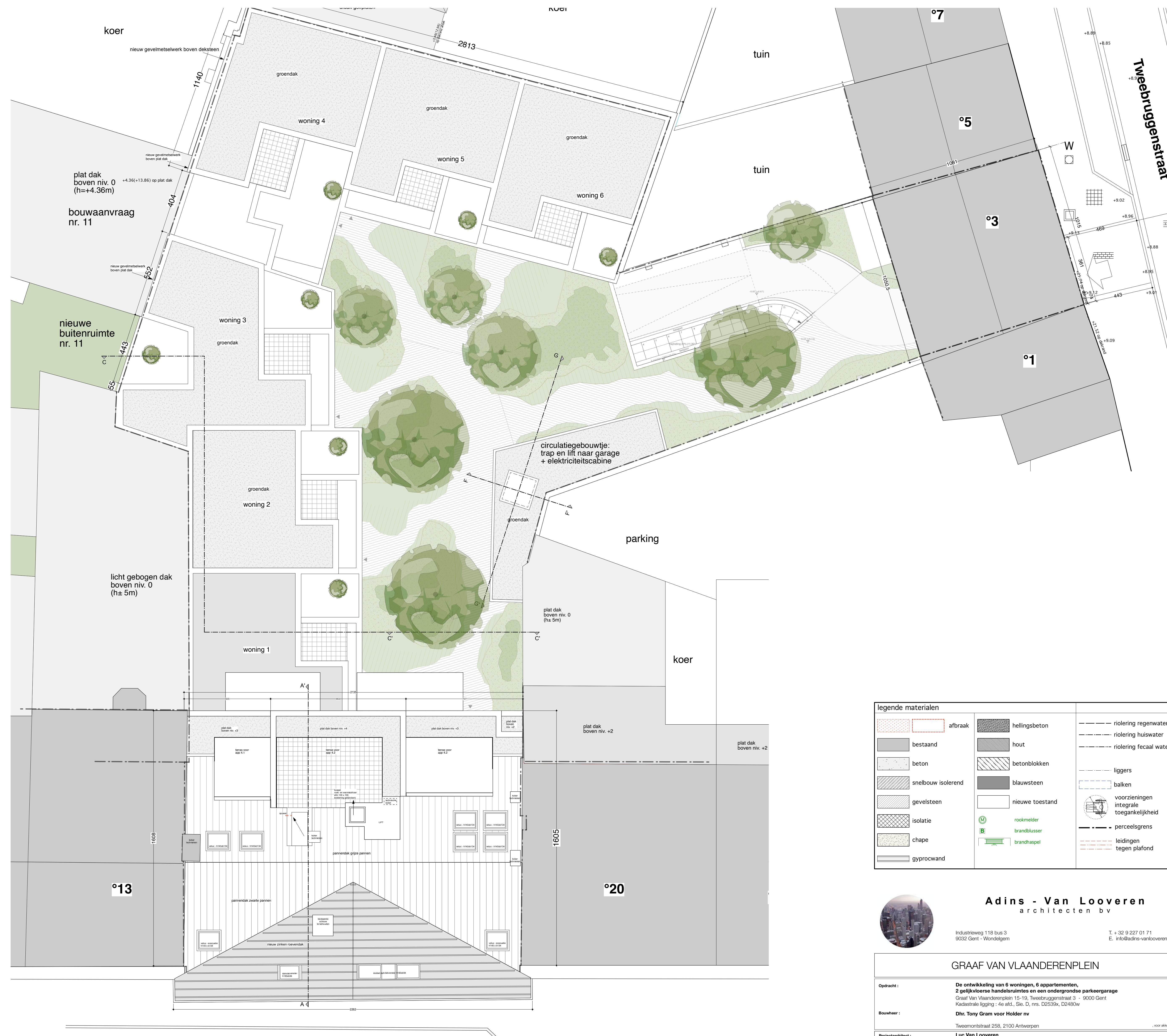
INPLANTINGSPLAN 1/100
