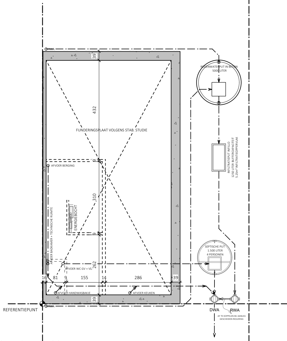
FUNDERINGS_ RIOLERINGSPLAN 1/100
