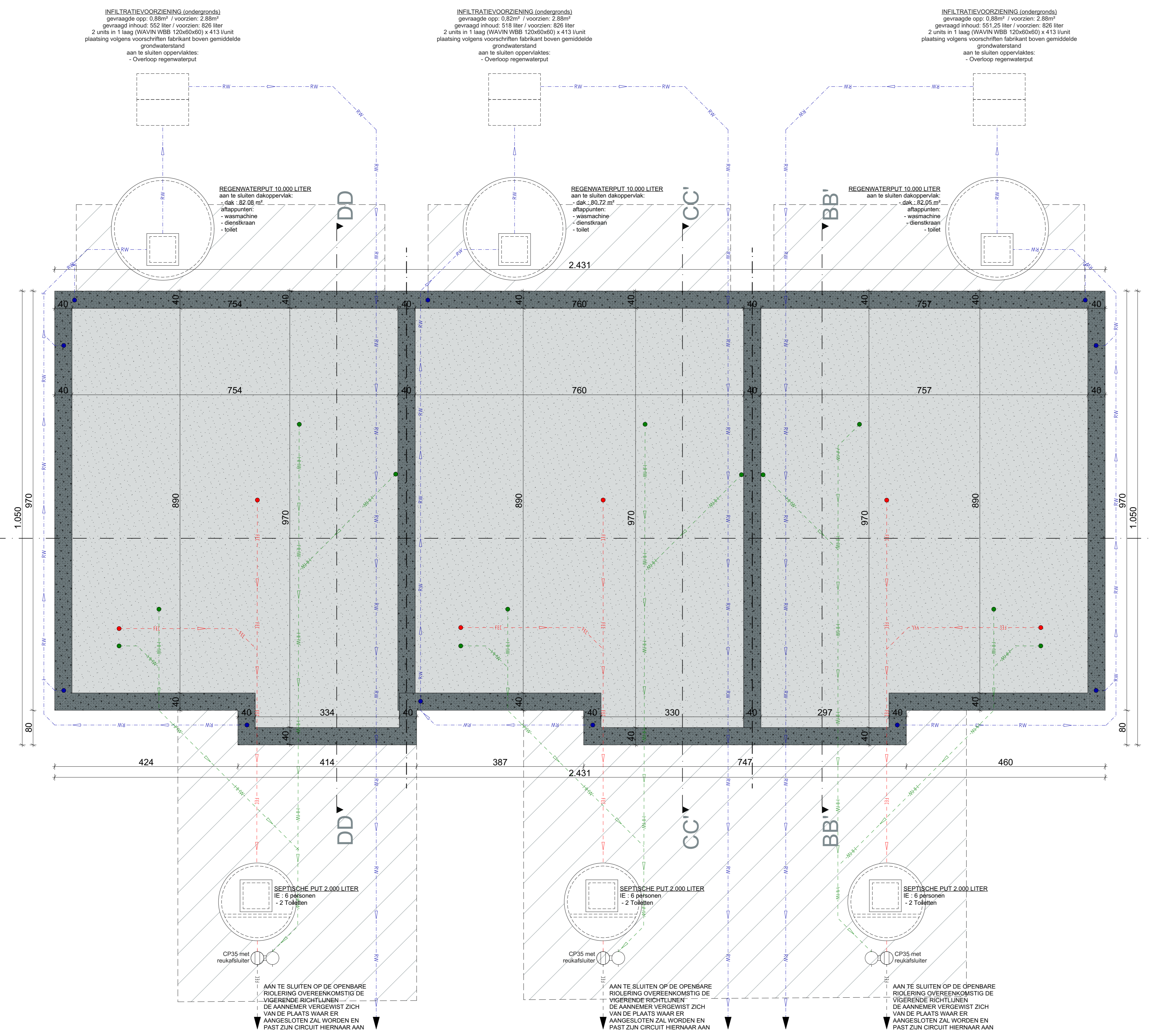
plan FUNDERING 1/50
