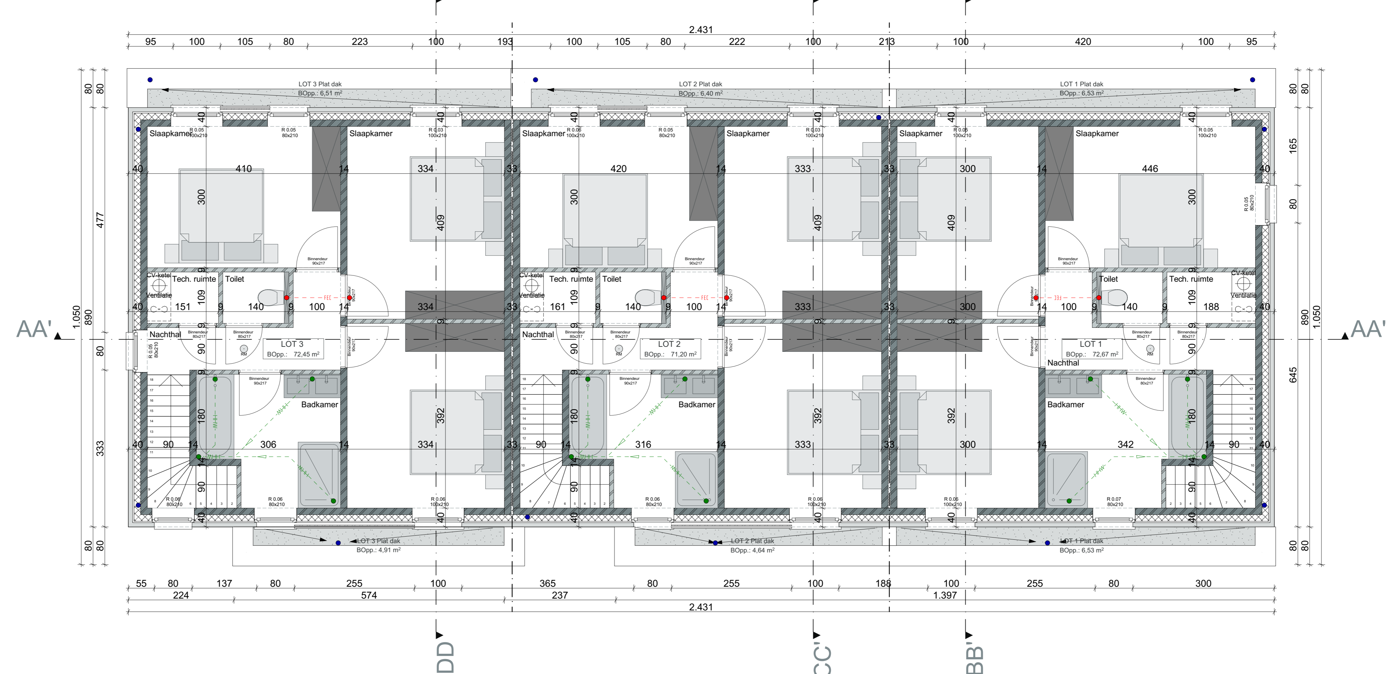
plan DAKENPLAN 1/50
