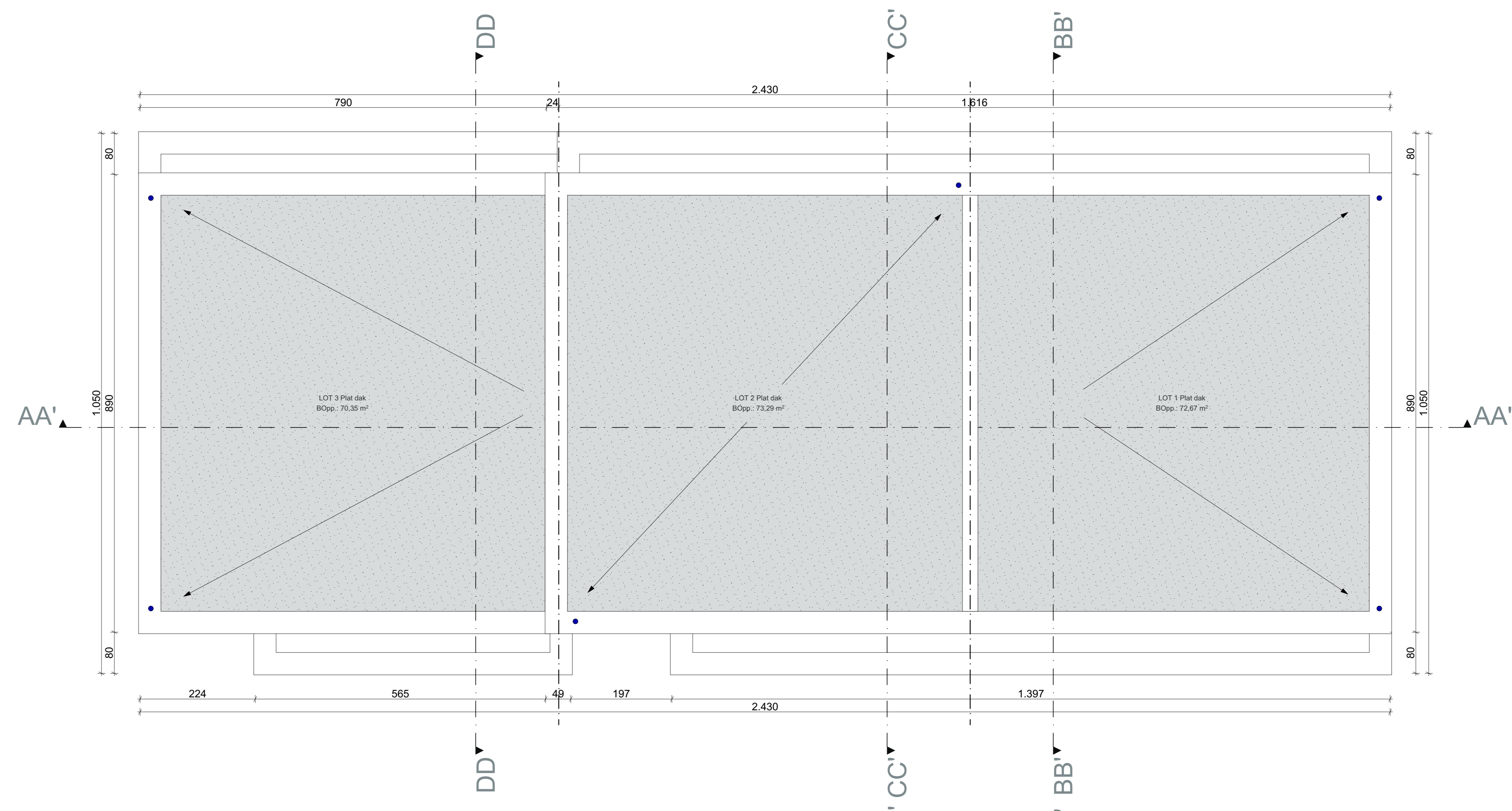
plan VERDIEPING +1 1/50
