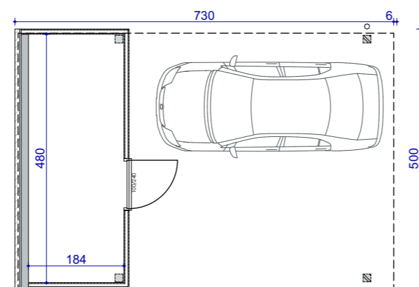
Carport/berging 1/100
