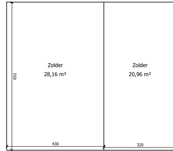
Zolder
