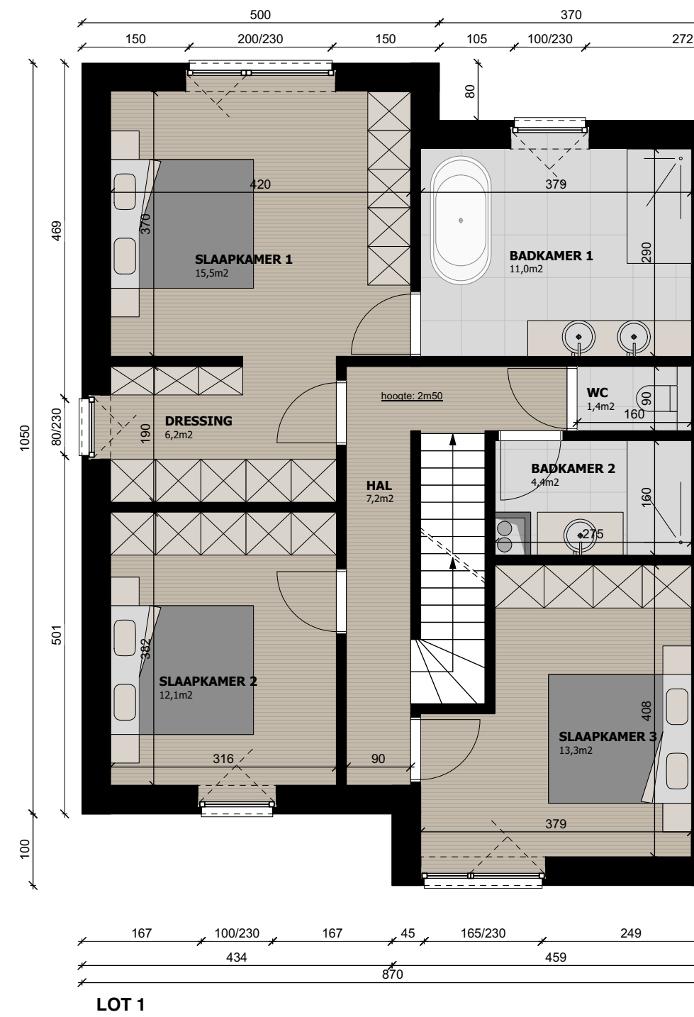
VERDIEPING 1/75
