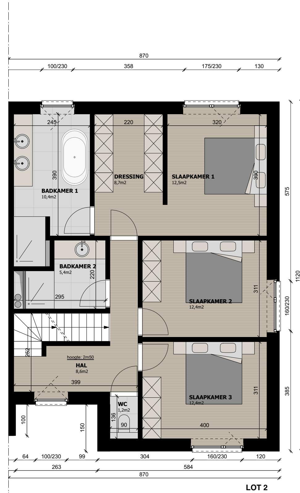
VERDIEPING 1/75
