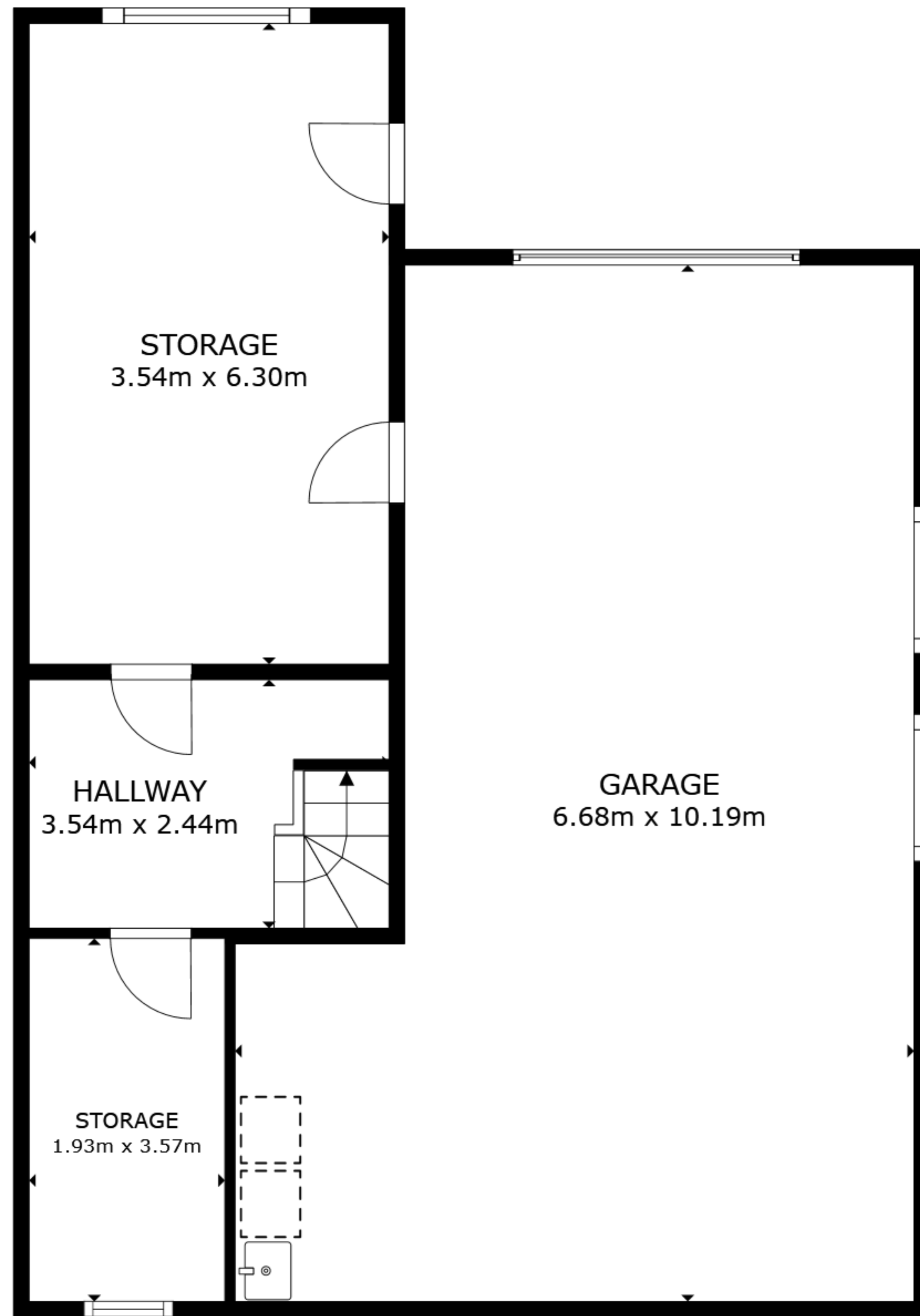
FLOOR 1
