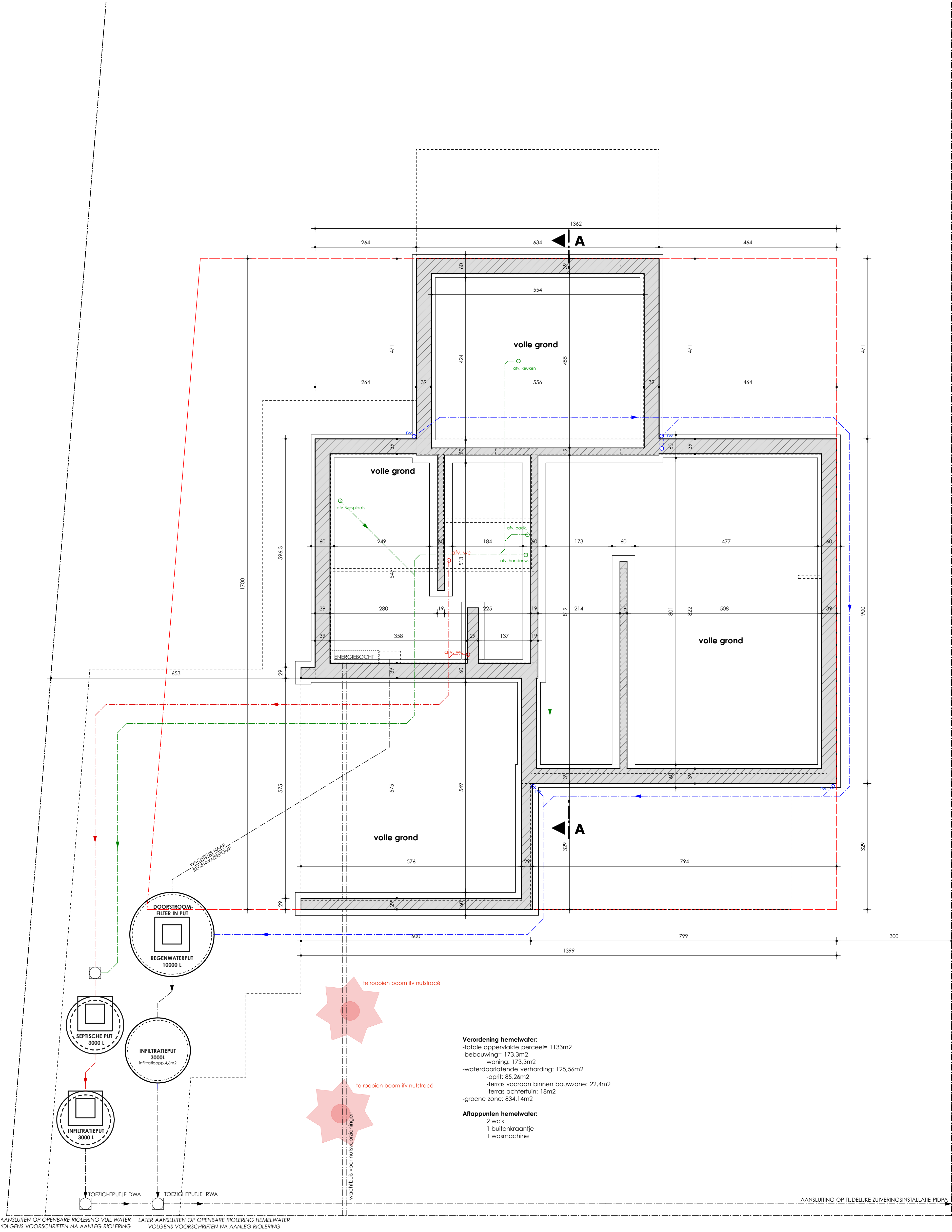
funderingsplan 1/50
