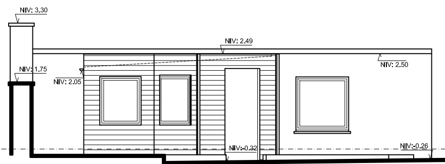
FACADE BB
