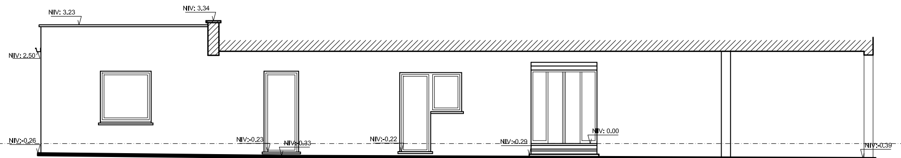
COUPE FACADE EE
