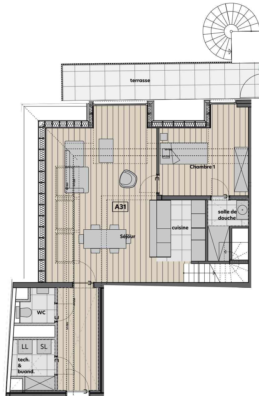
Plan R+3 1/100
