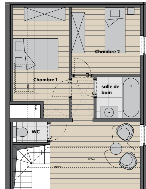
Plan R+4 1/100
