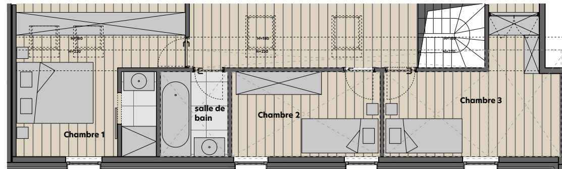
Plan R+4 1/100
