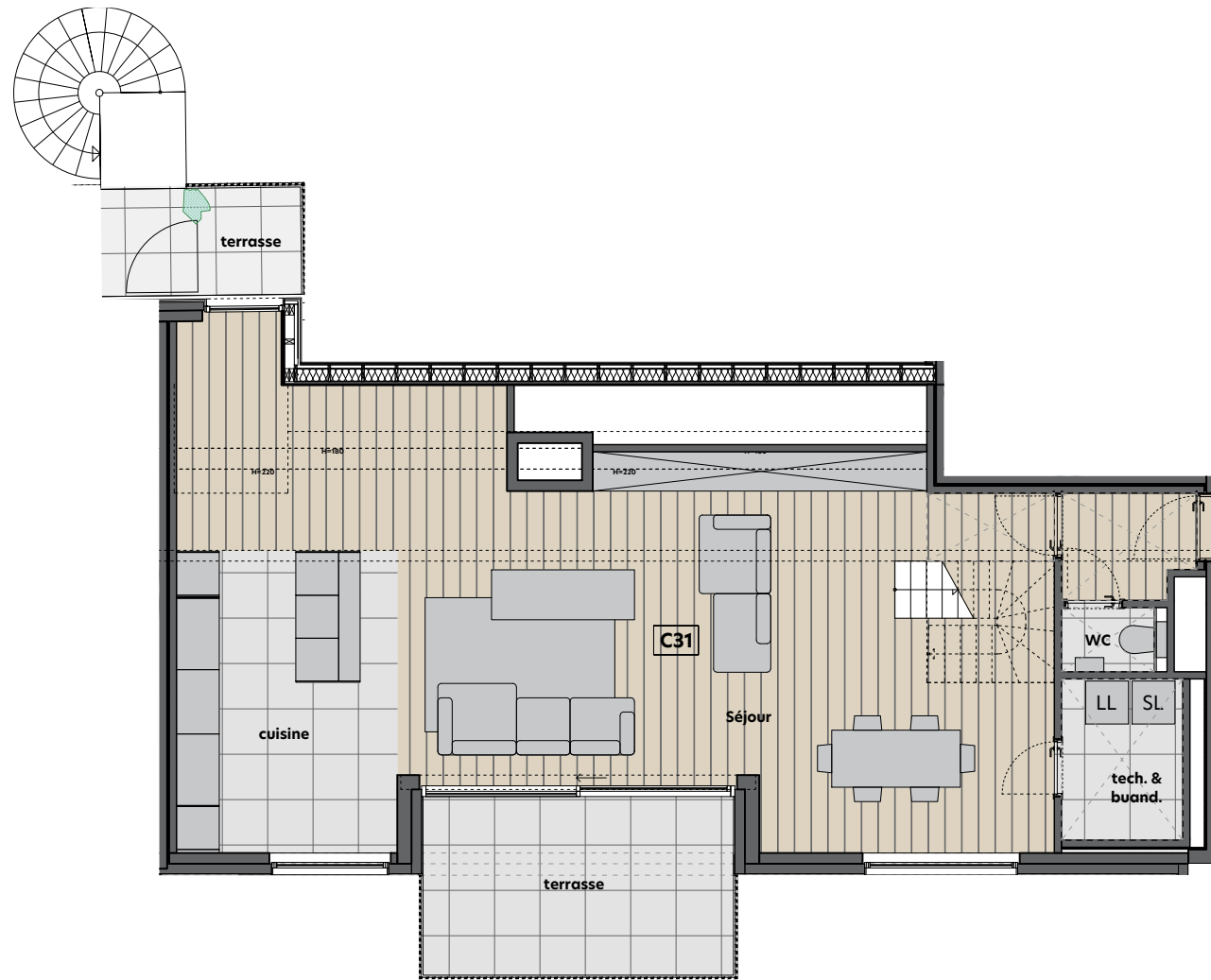
Plan R+3 1/100
