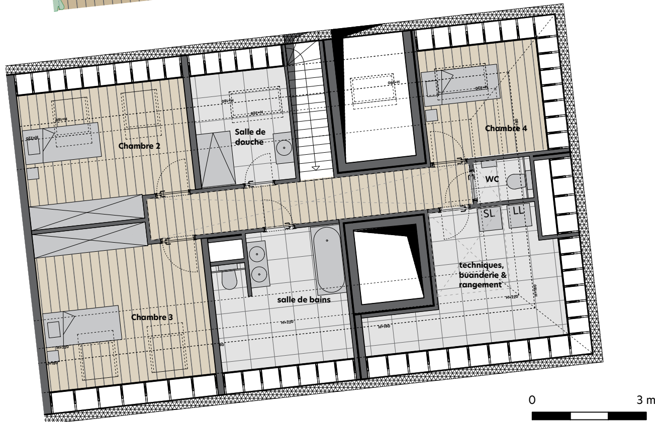
Plan R+4 1/100
