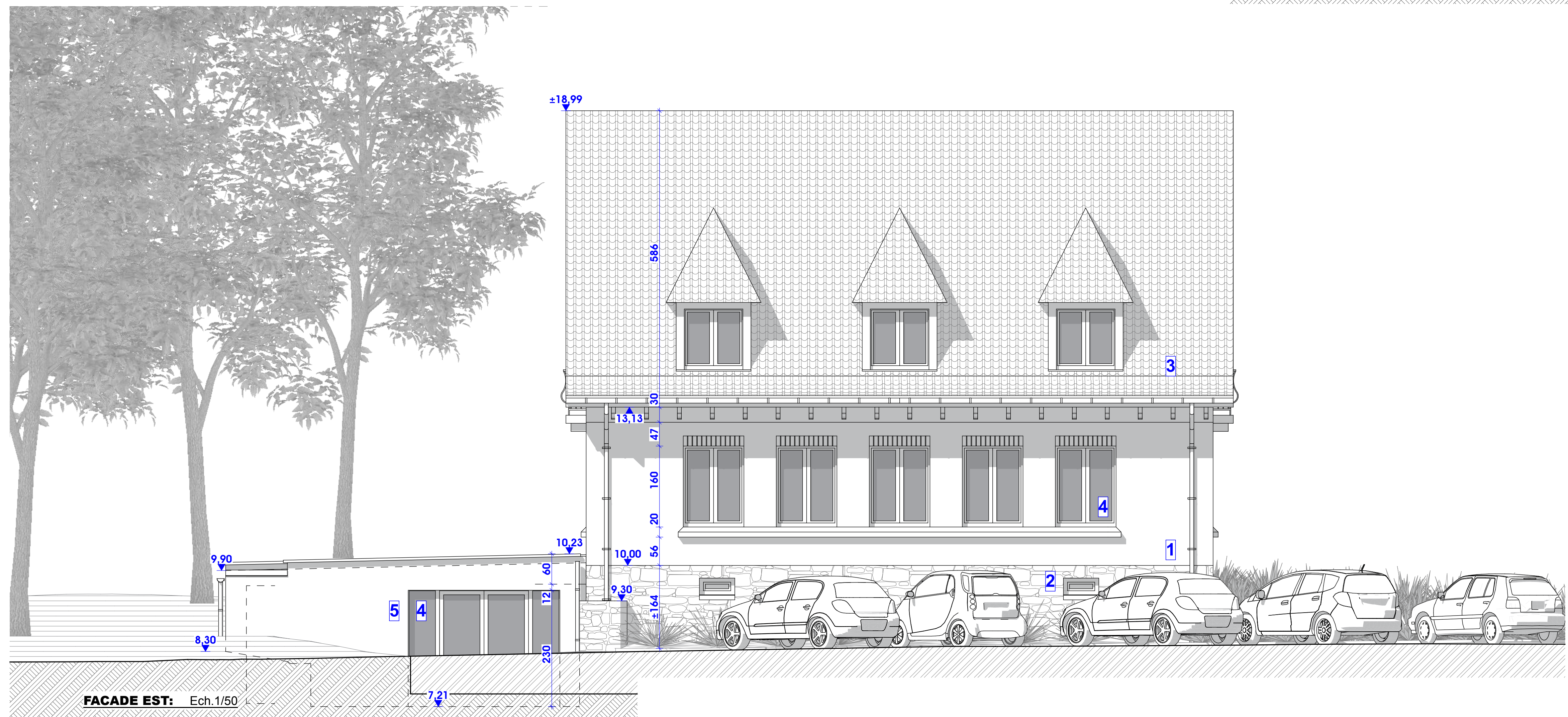
FACADE OUEST: Ech. 1/50
