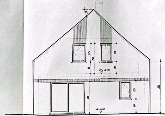
FACADE ARRIERE Ech. 1/50
