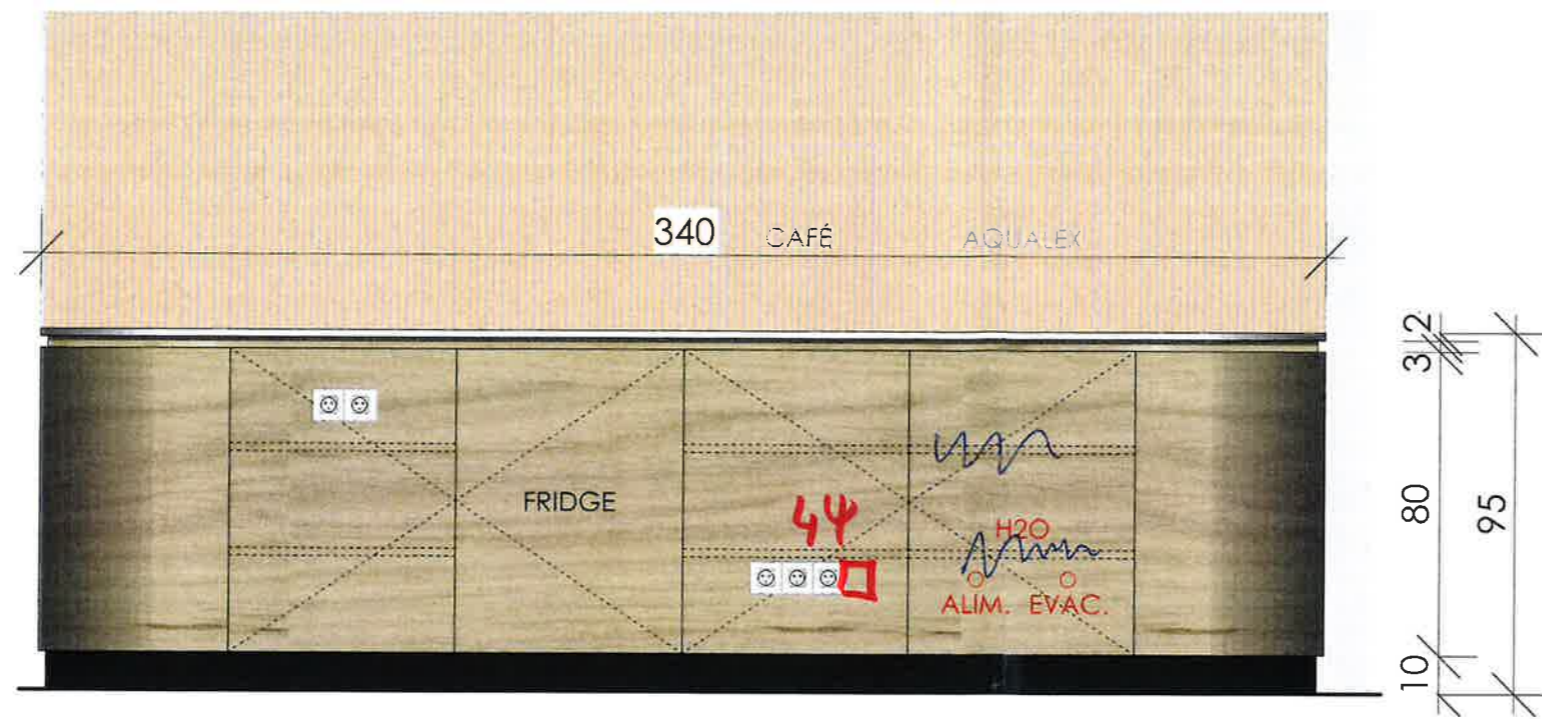
ELEVATIONS
