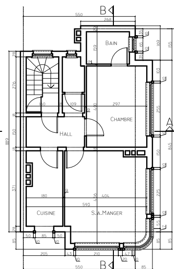
2 EME ETAGE (Existant)
